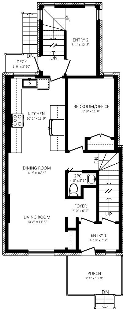
MAIN FLOOR 918 SQUARE FEET APPROX. 8'6" CEILING
