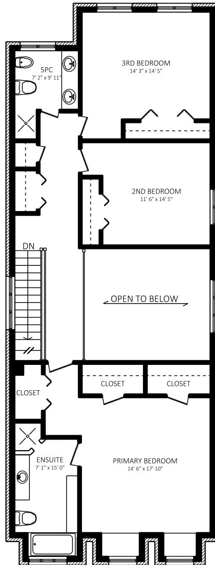
SECOND FLOOR 1300 SQUARE FEET APPROX. 8' CEILING HEIGHT
