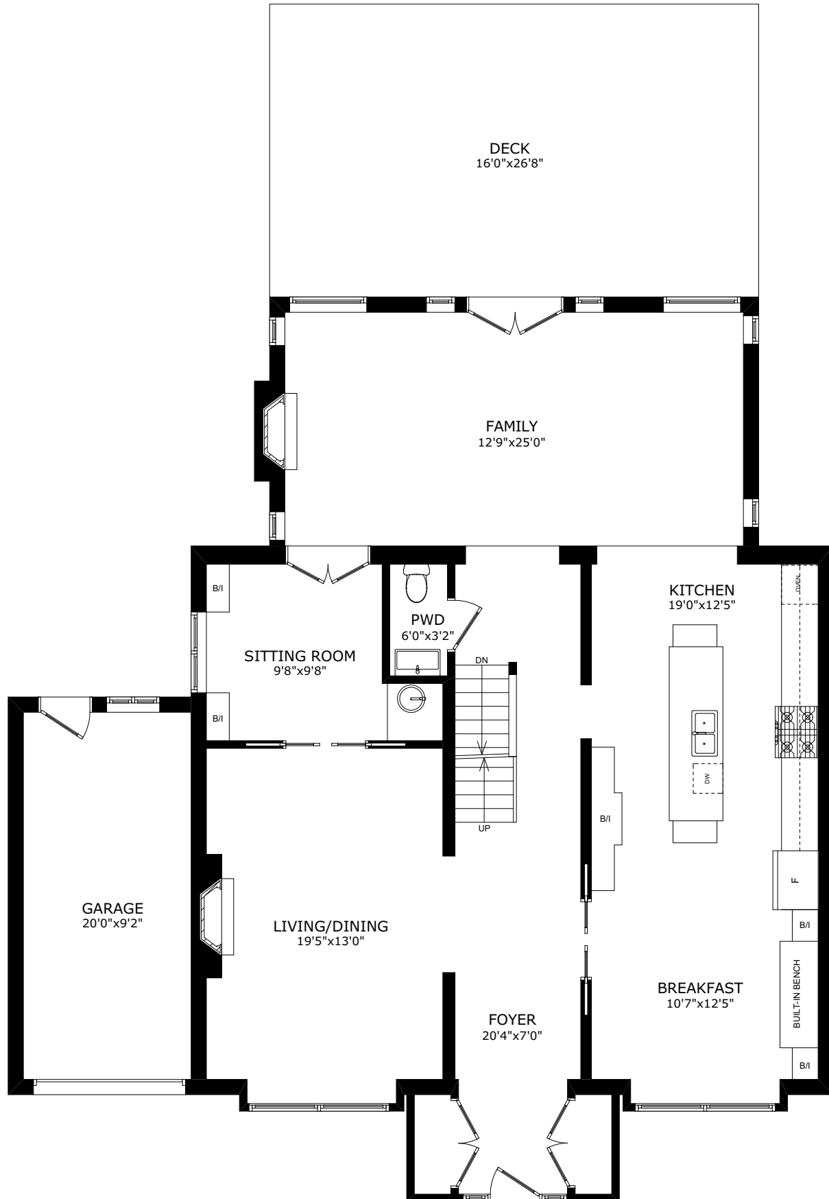
MAIN FLOOR
